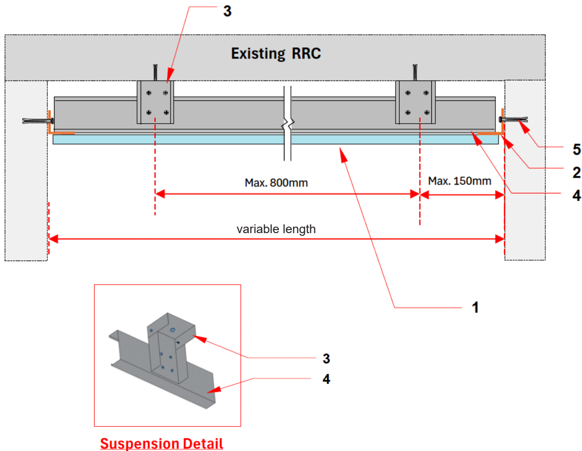
« Ceiling Linear - 1 x 13 GM on one side of a 50 UC Frame »
