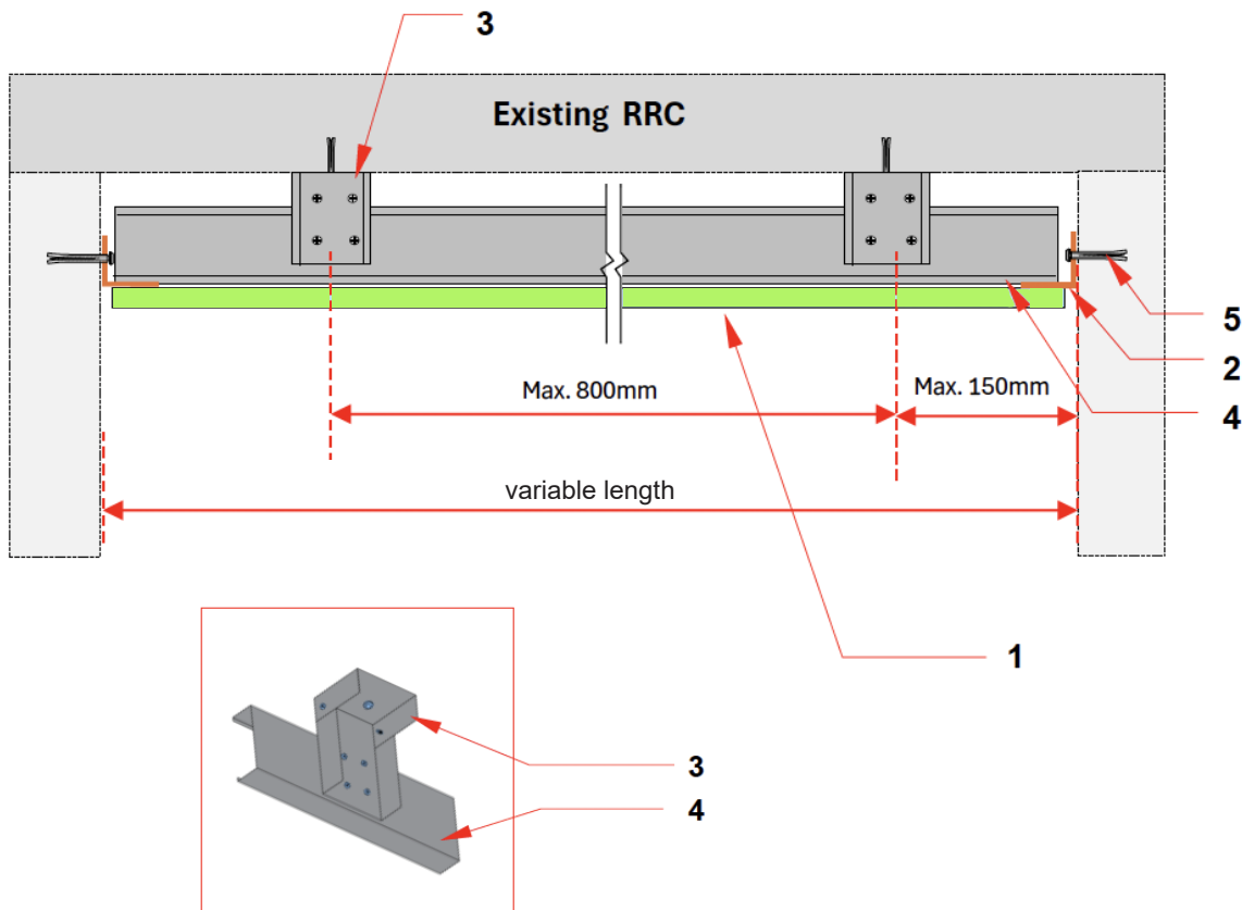
Suspension Detail
