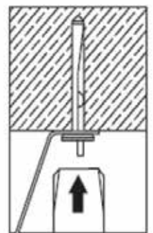
Hammer in anchor.
