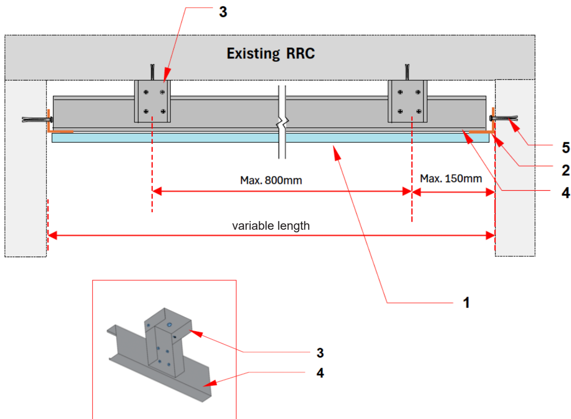
Suspension Detail
